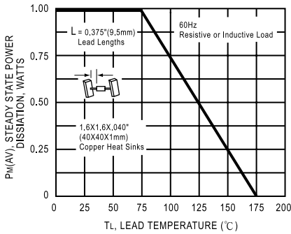
FIG. 5 - STEADY STATE POWER DERATING CURVE
